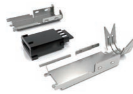
DG1106 Series IEEE 1394 6 Positions Male Solder Type
